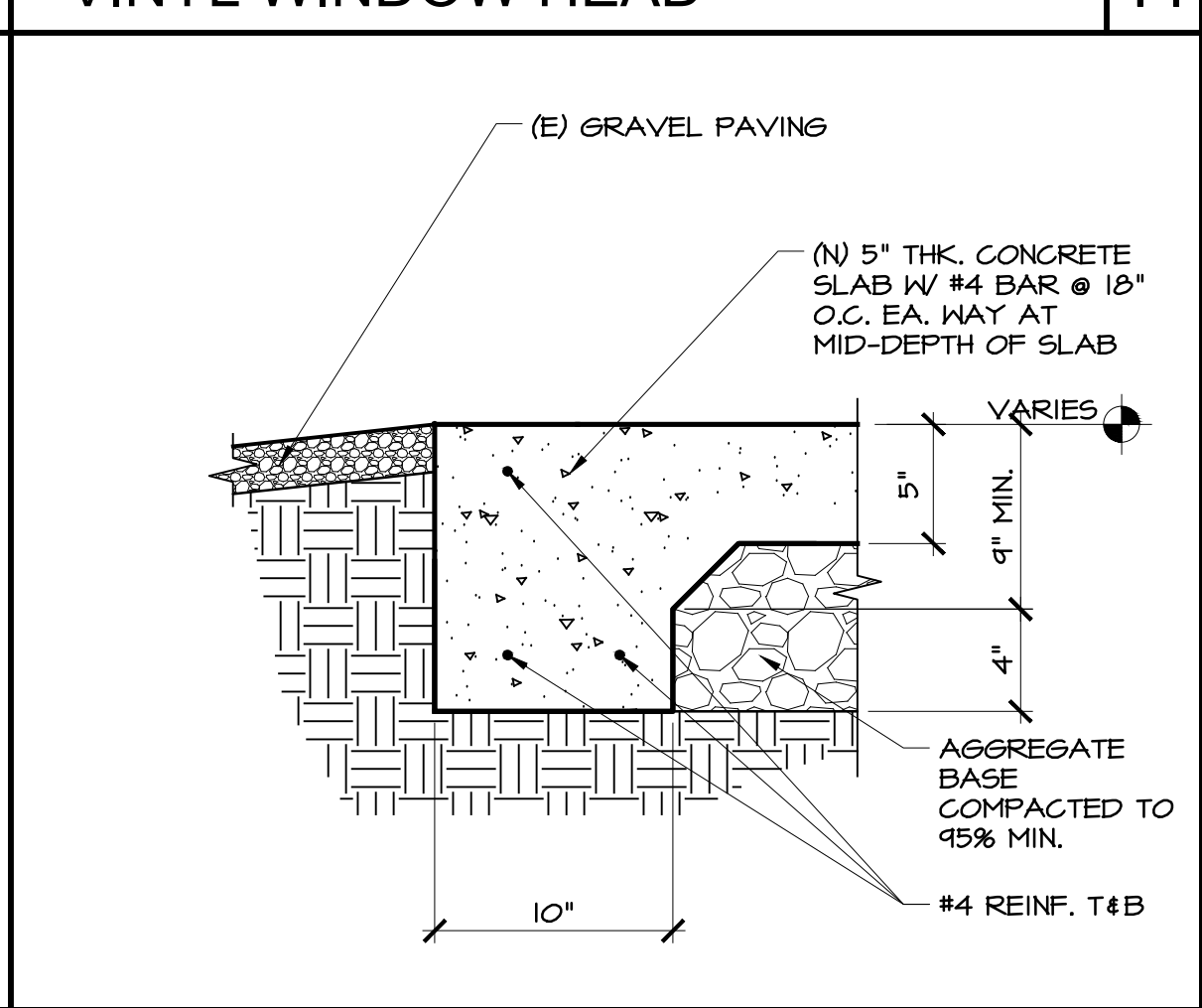
(N) CONCRETE PARKING SLAB 1 1/2"=1'-0" 15
