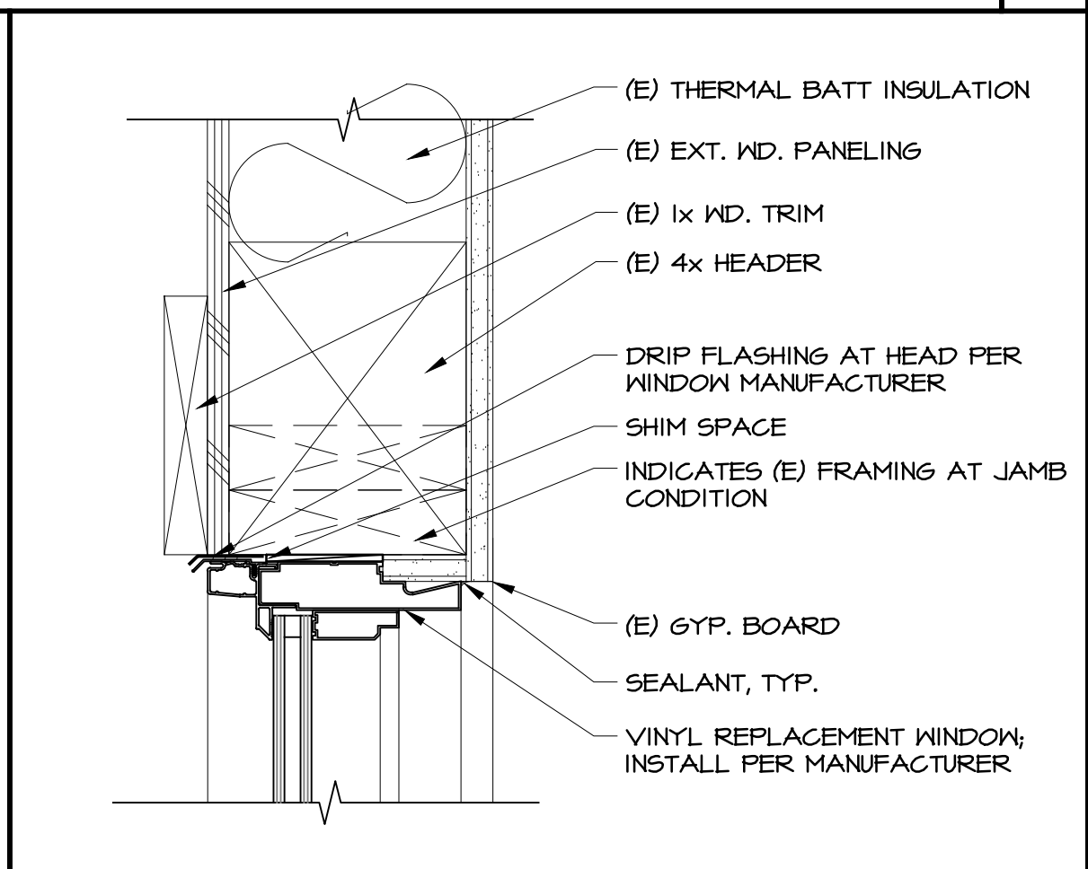
VINYL WINDOW HEAD (JAMB SIM) 3"=1'-0" 14
