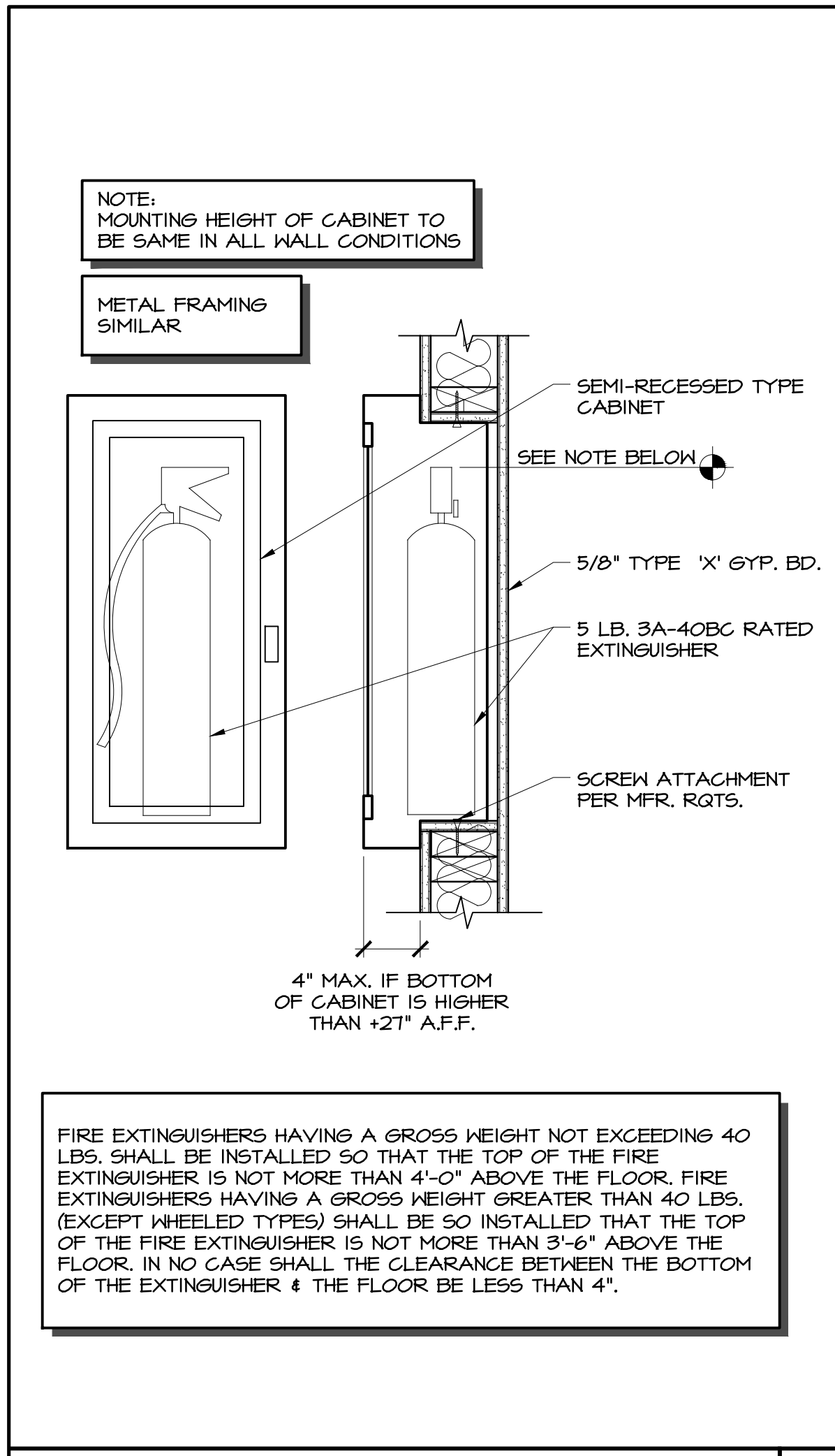
SEMI-RECESSED F.E. CABINET 1 1/2"x1'-0" 18
