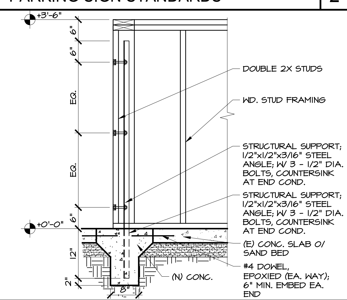
SUPPORT @ PARTIAL WALL 3/4" = 1'-0" 3
