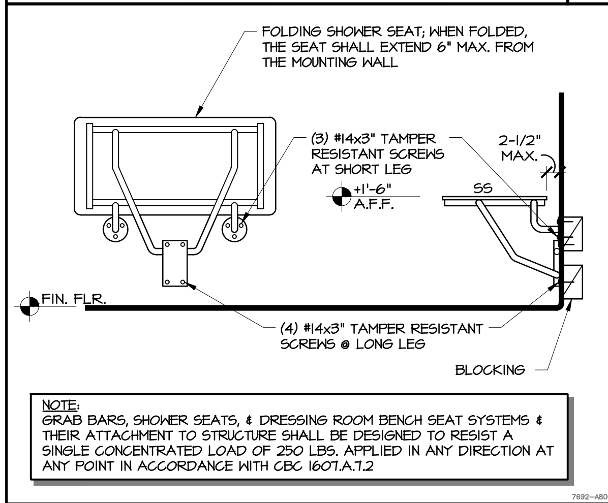
ACCESSIBLE SHOWER SEAT 3/4"x1'-0" 19
