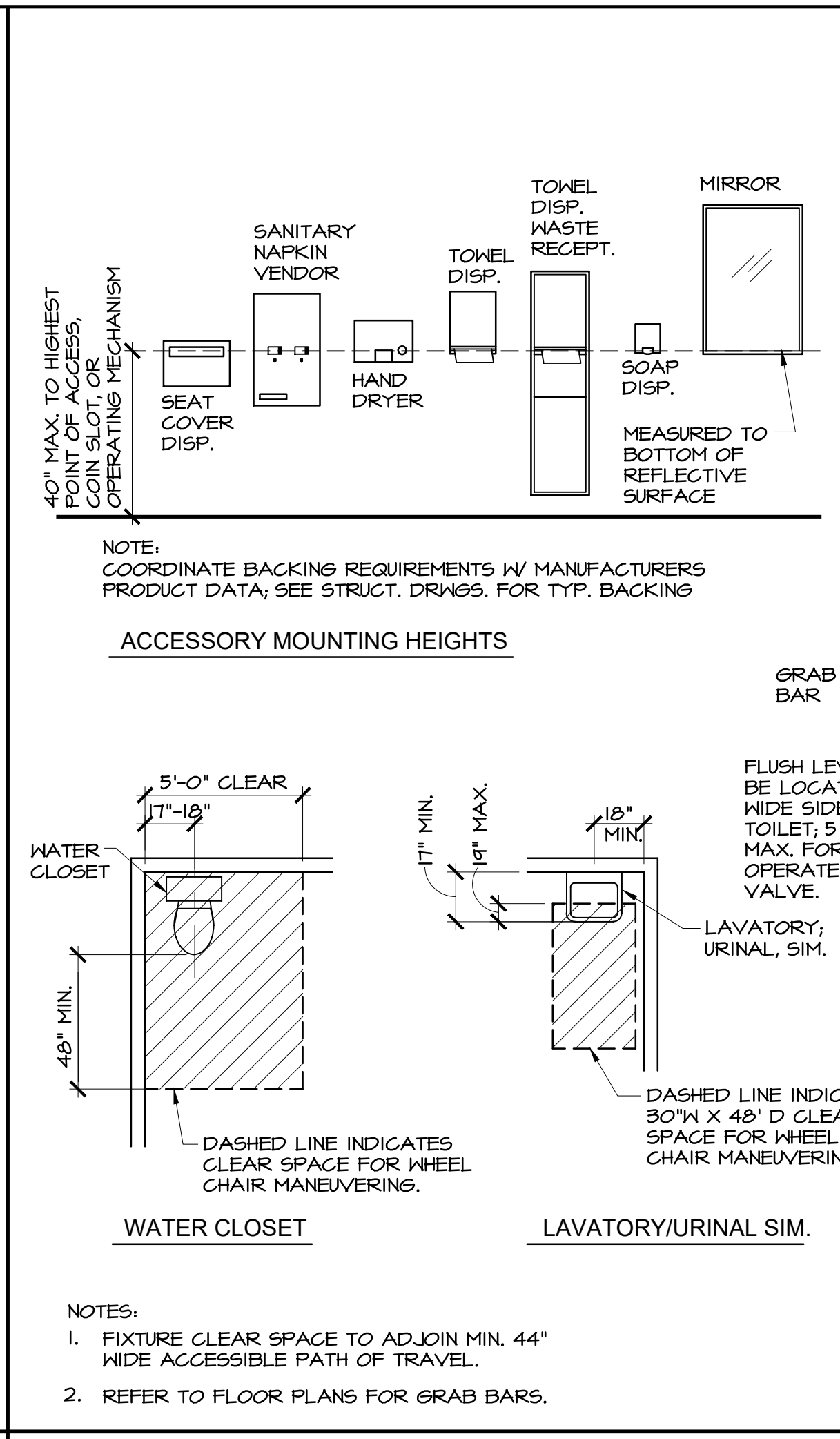
TYPICAL ACCESSIBLE FIXTURE CLEARANCES & MOUNTING HEIGHTS N.T.S. 10
