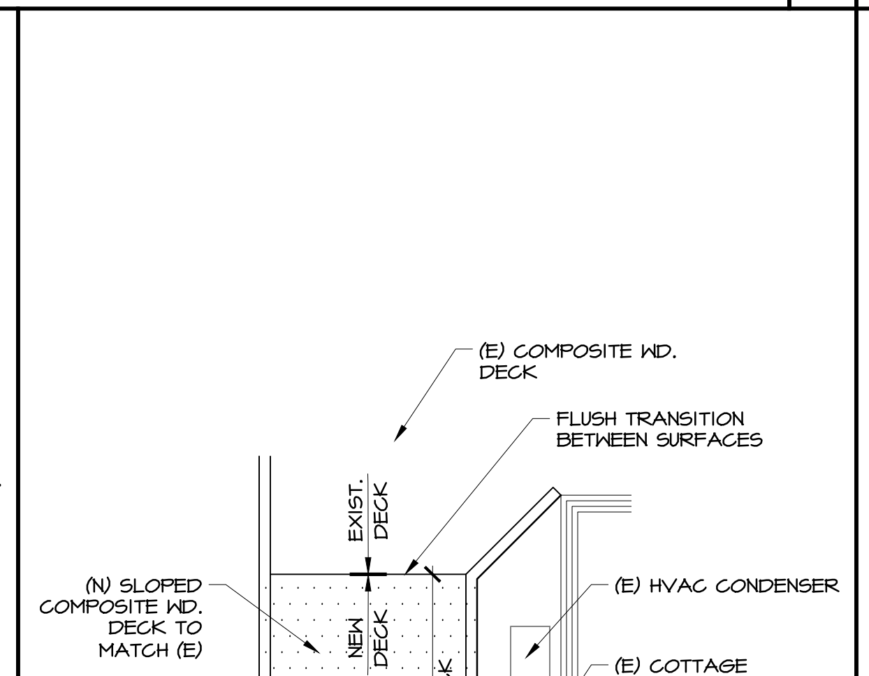
(N) SLOPED DECK 1/4"=1'-0" 7
