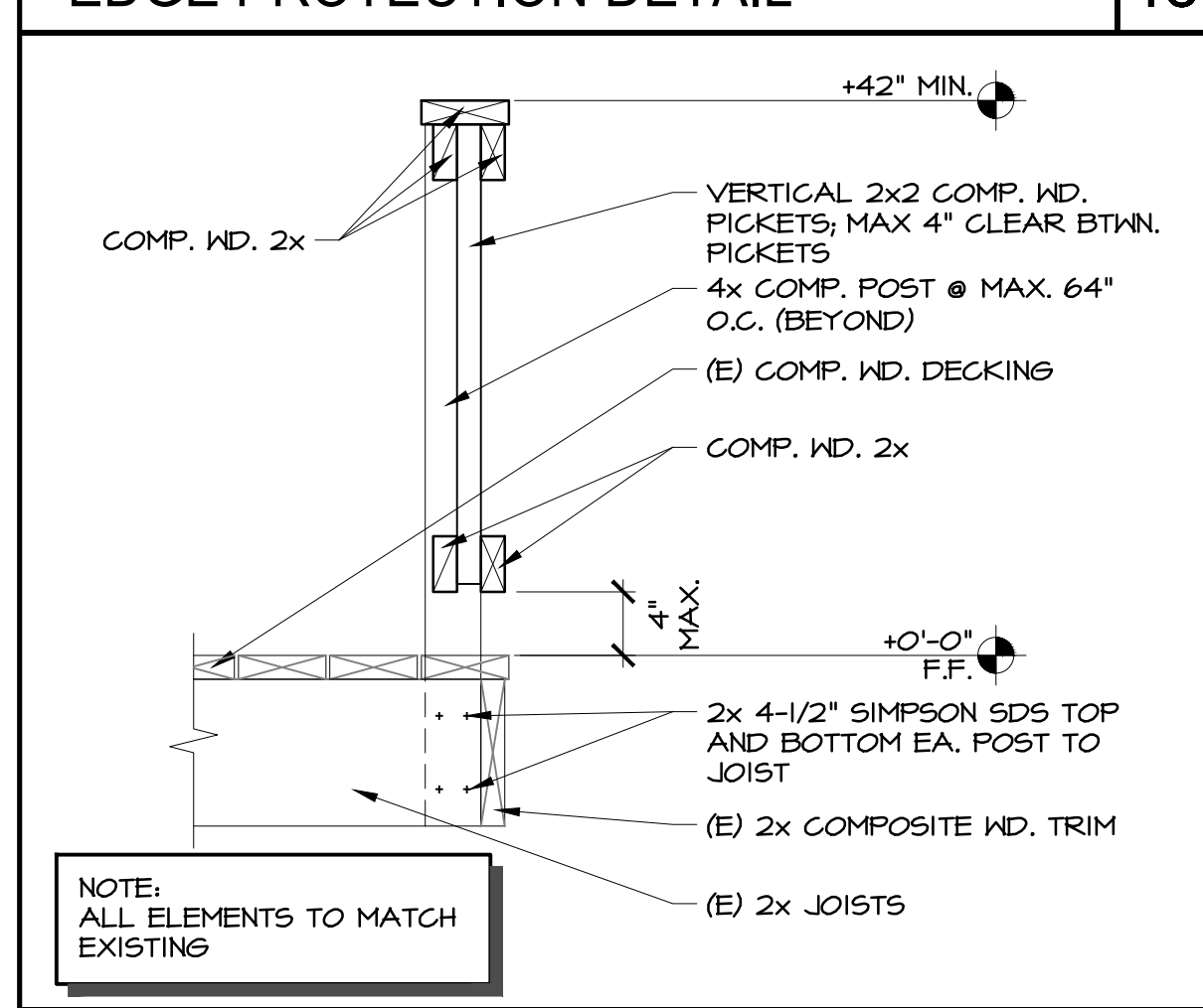
GUARDRAIL DETAIL 1/4"=1'-0" 19
