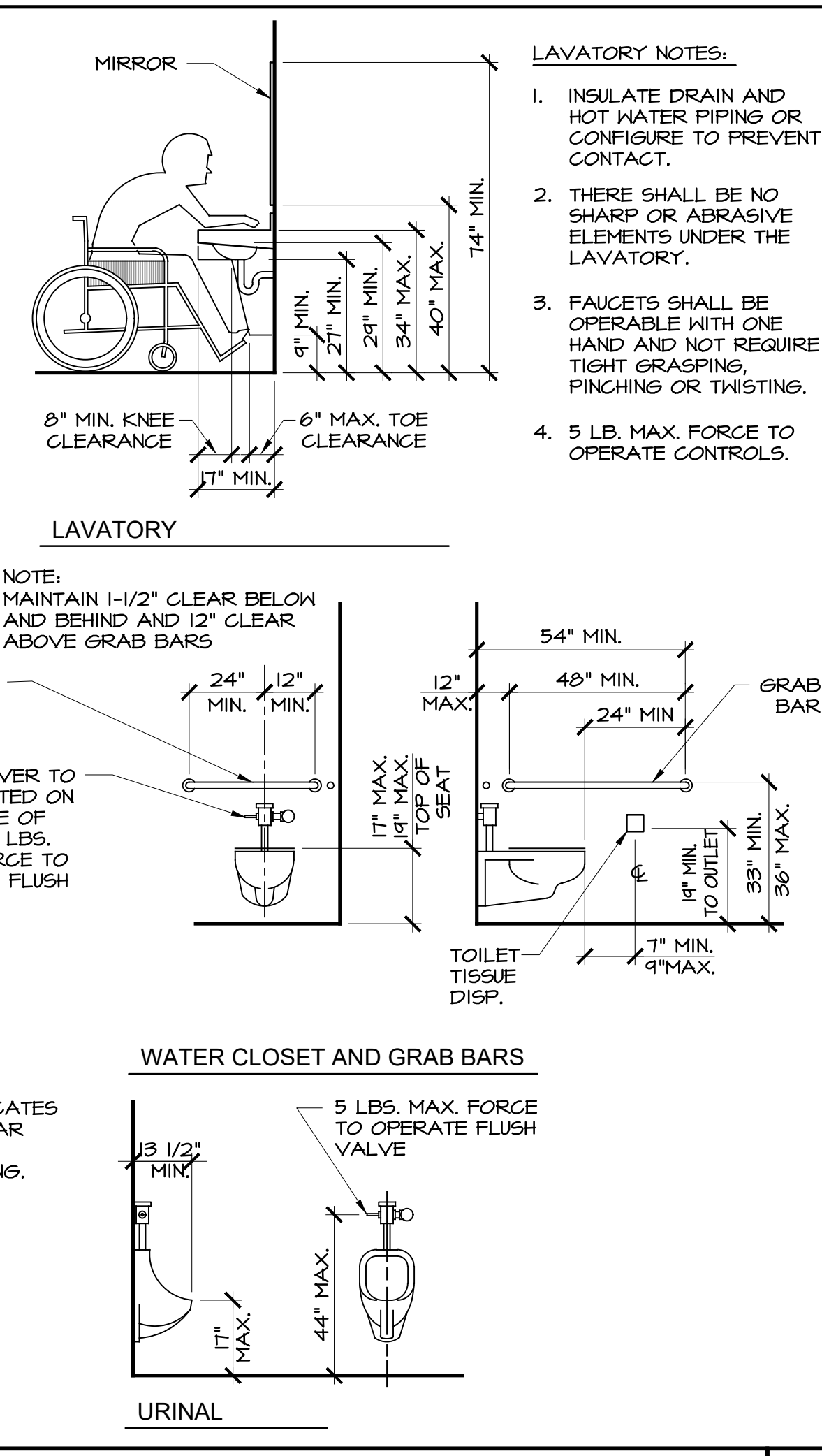
TYPICAL ACCESSIBLE FIXTURE CLEARANCES & MOUNTING HEIGHTS N.T.S. 10
