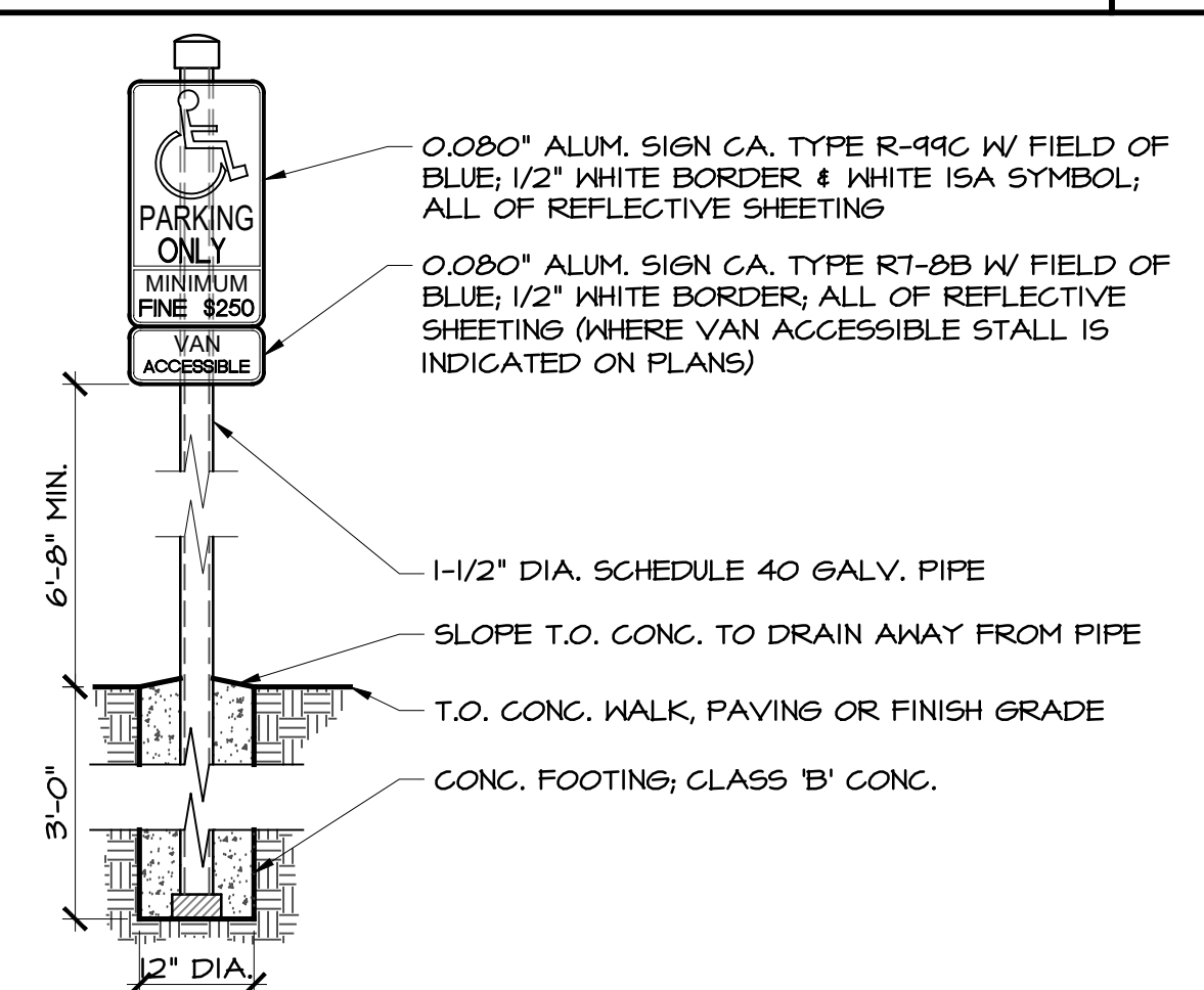
PARKING SIGN STANDARDS N.T.S. 2
