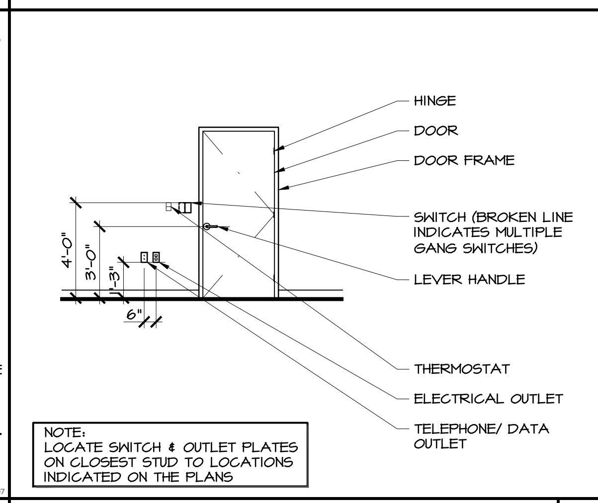
TYP. MOUNTING HEIGHTS N.T.S. 8
