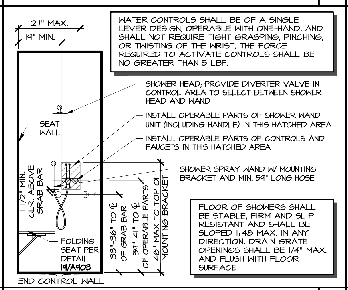
ACCESSIBLE SHOWER ELEVATION 1/2"x1'-0" 16
