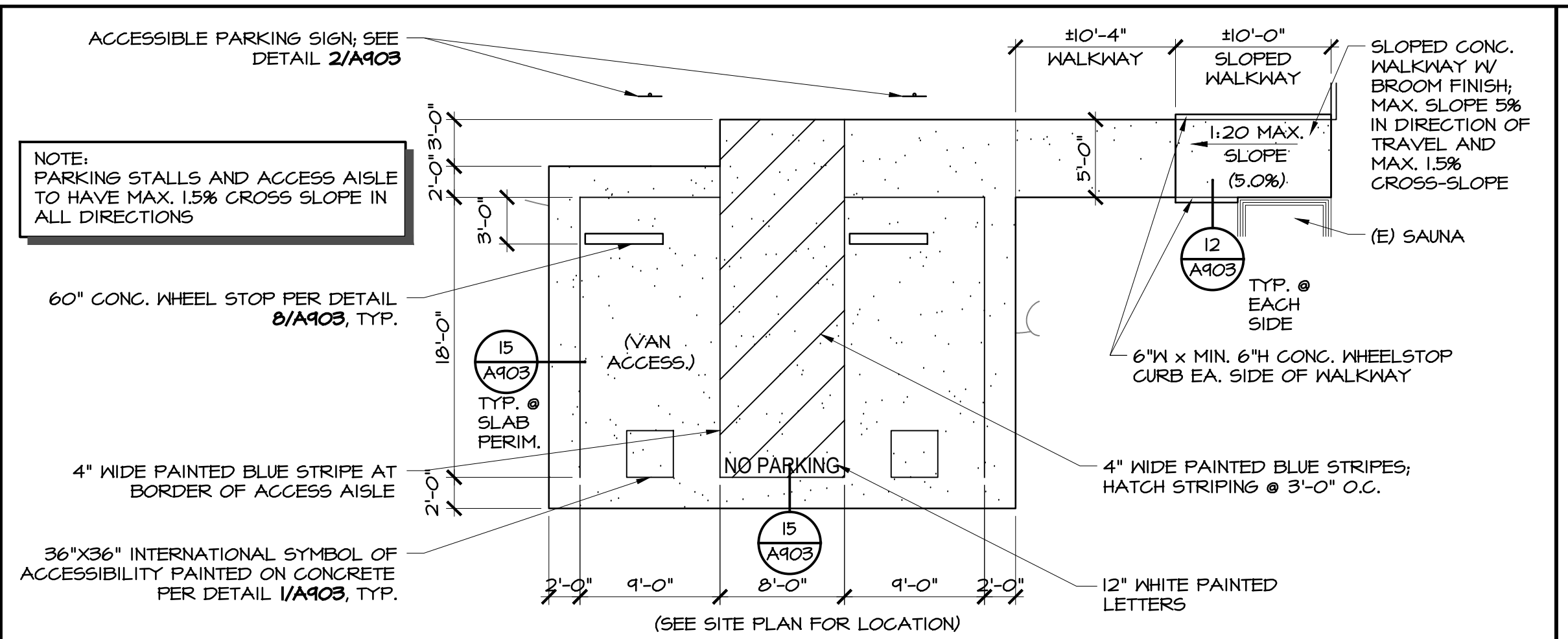
VAN ACCESSIBLE PARKING STALLS 1/8"=1'-0" 5
