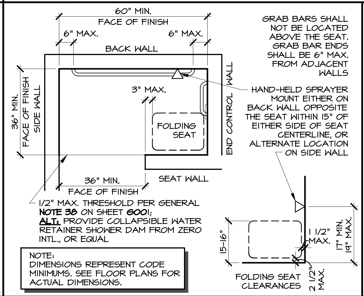
ACCESSIBLE SHOWER PLAN 1/2"x1'-0" 15
