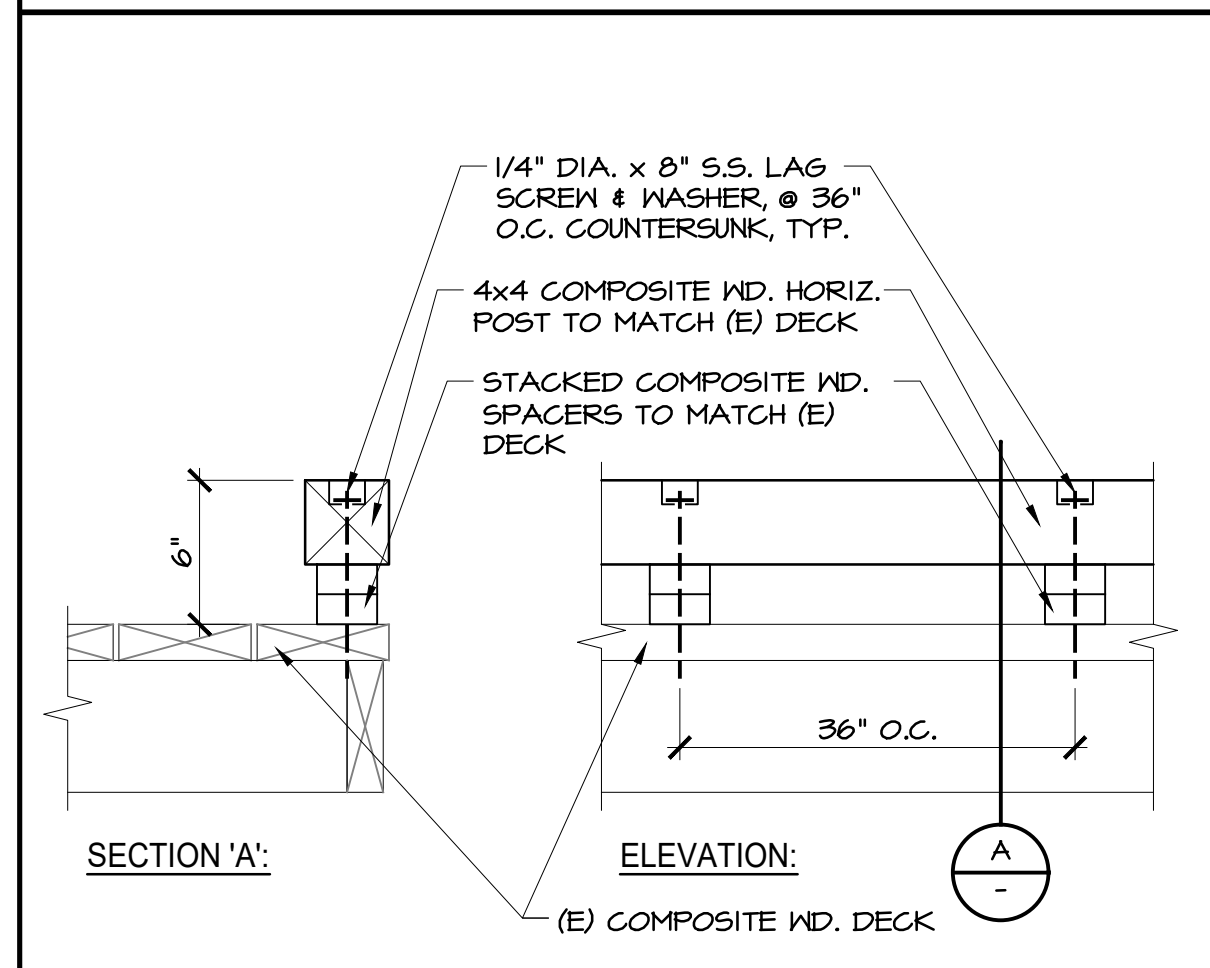
EDGE PROTECTION DETAIL 1 1/2"=1'-0" 18
