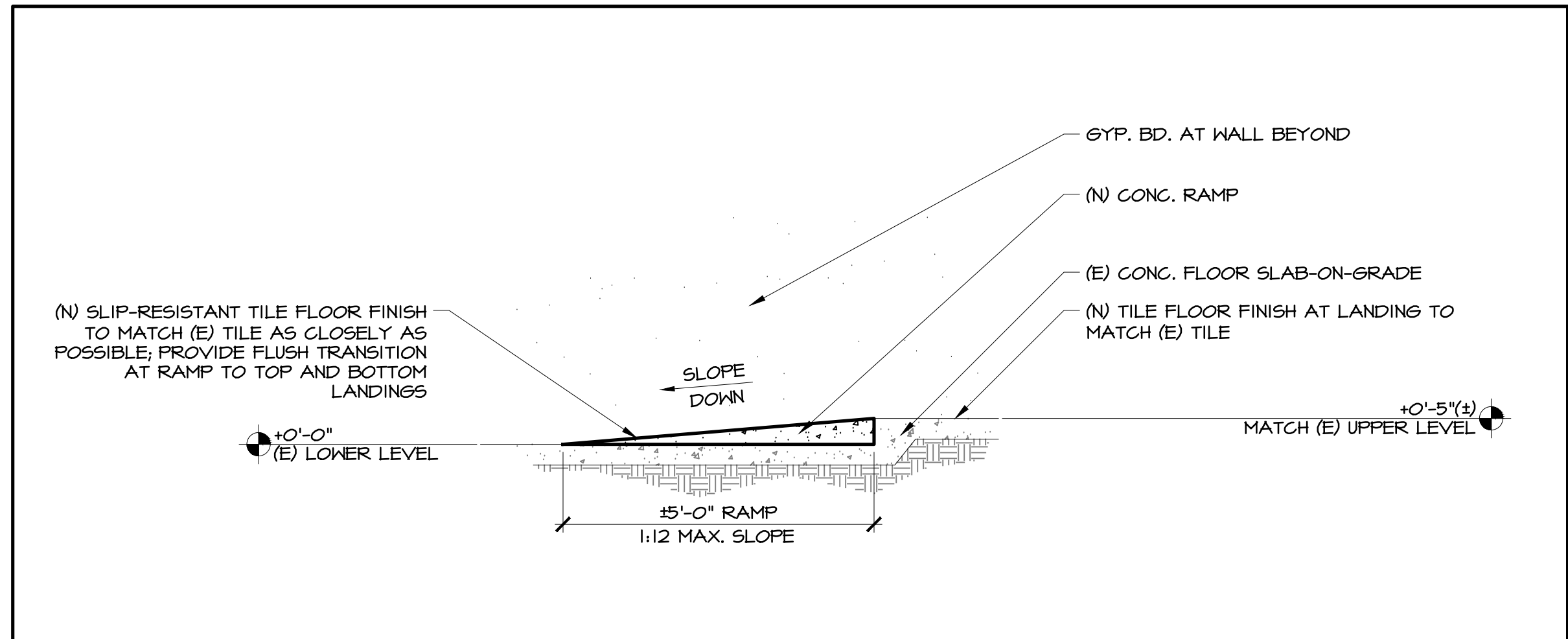
(N) RAMP SECTION 1/2"=1'-0" 13
