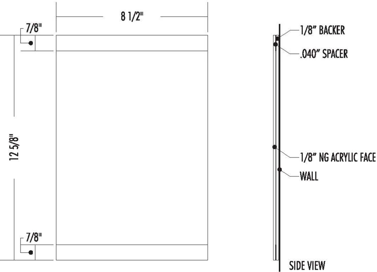
SIGN TYPE 22C
