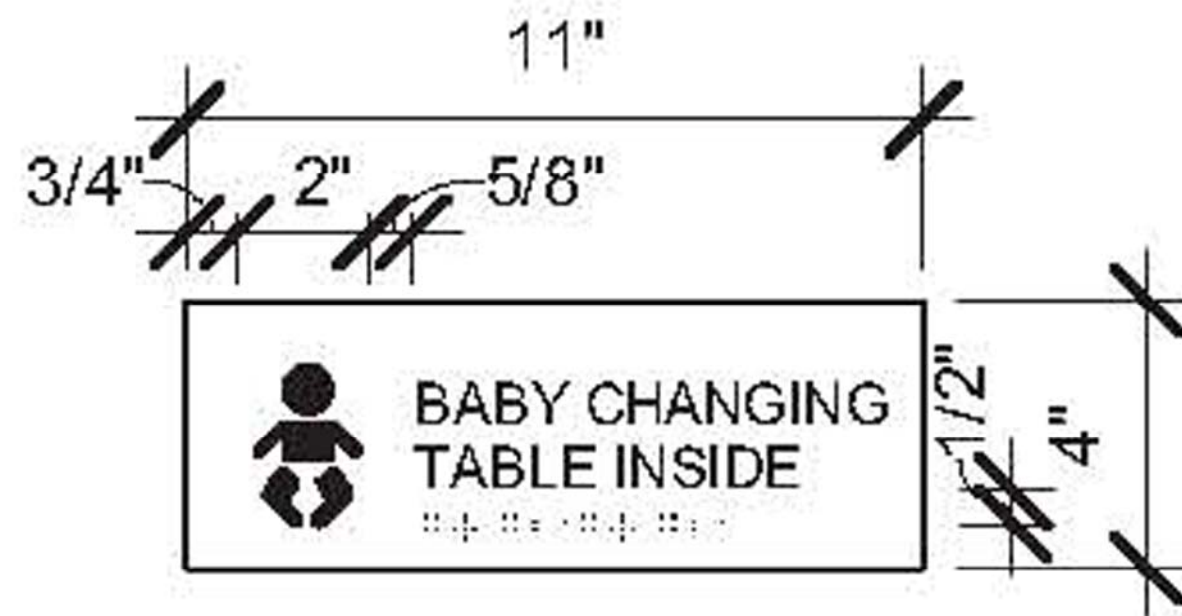
SIGN TYPE I5A
