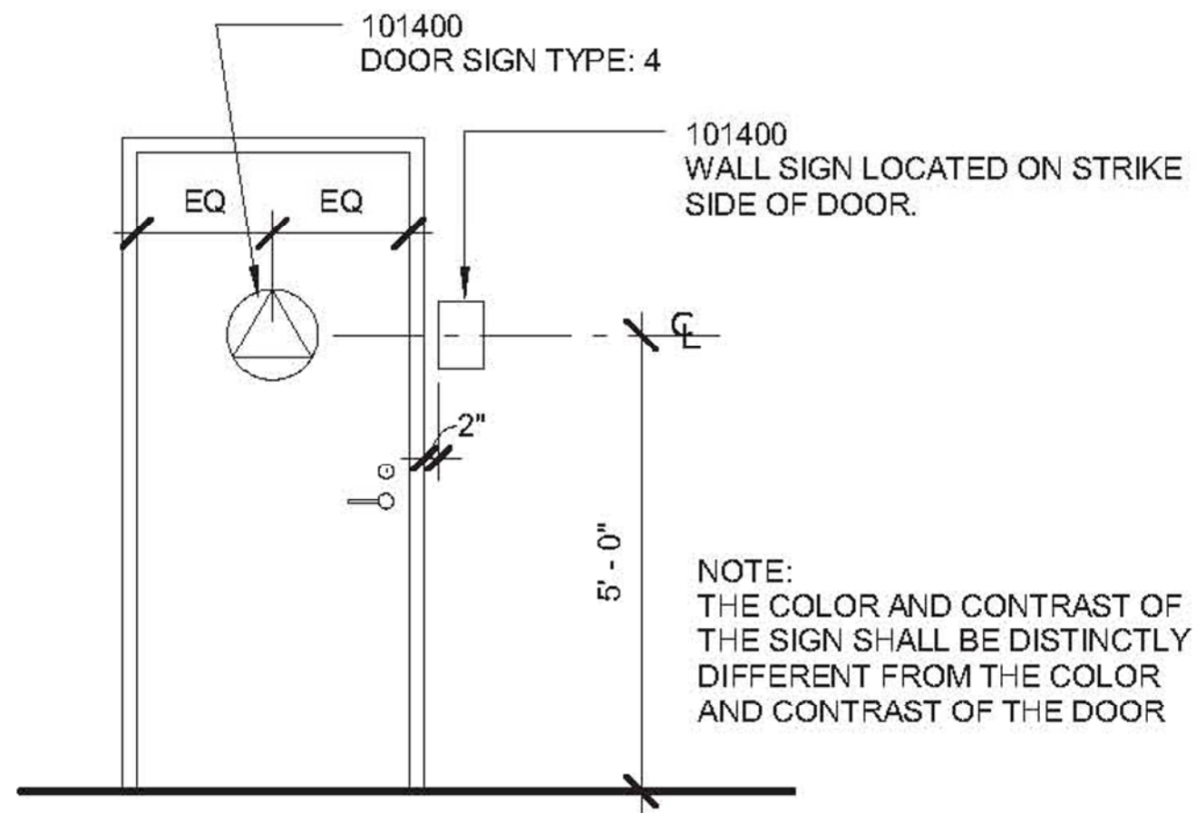
Typical Mounting Locations
